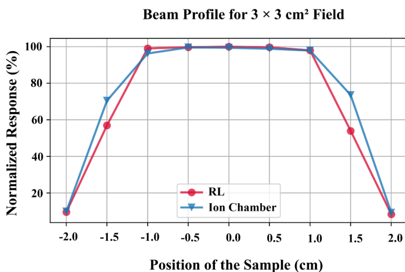
Figure 5. Comparison of the transverse profile obtained on a 3 \times 3 cm 2 6 MV photon beam using Ge optical fiber and CC-13 ion chamber, whereas the position of the sample range spans from -2.0 cm to +2.0 cm, and nine times repetition of measurement in different positions.
