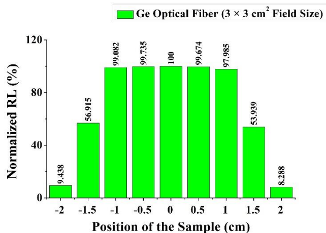
Figure 3. Transverse beam profile of a 3 \times 3 cm 2 small field using Ge optical fiber, whereas the position of the sample range spans from -2.0 cm to +2.0 cm, and nine times repetition of measurement in different positions.
