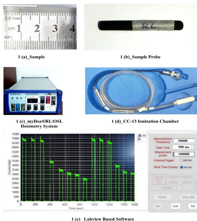
Figure 1. Graphical represents a) the sample of Ge optical fiber, b) sample probe, c) myDoz®RL/OSL Dosimetry System for RL signal measurements, d) CC-13 ion chamber for dose measurements, e) Labview based software interface for data acquisition.
